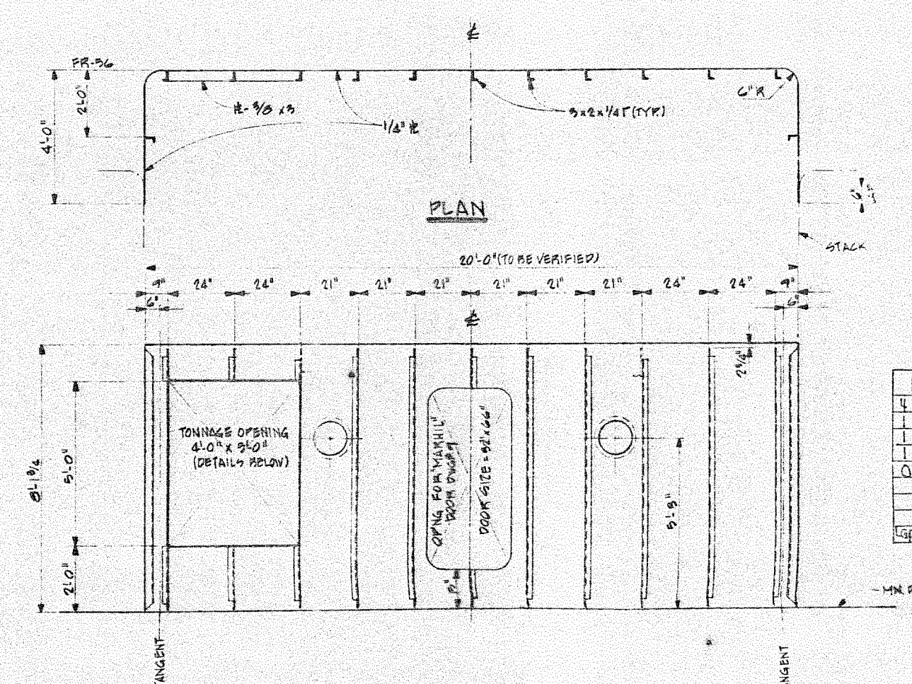
AFT BULKHEAD-LOOKING AFT SCALE 1/2" = 1'-0"
