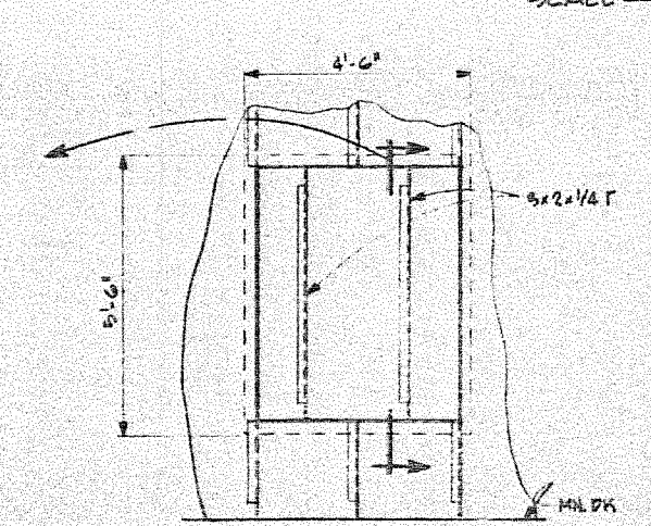
DETAILS TONNAGE OPENING SCALE 1/2" = 1'-0"
